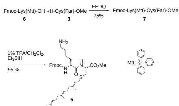
Scheme 3. Removal of the methyltrityl group in the presence of a farnesyl moiety.
