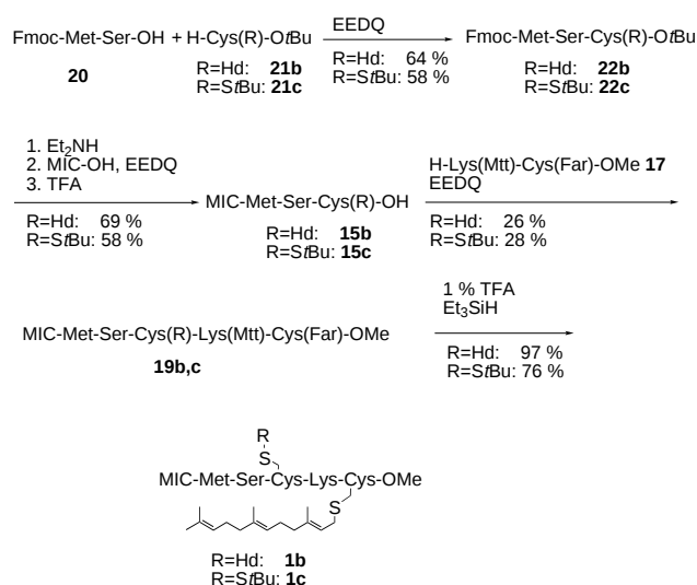
Scheme 7. Synthesis of the analogous peptides 1b and 1c by the Mtt strategy.
