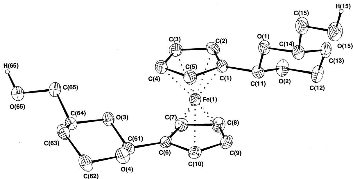
Fig. 1. Cameron view of the molecule with ellipsoids plotted at the 50% probability level. Hydrogen atom but those attached to the hydroxy group have been omitted for clarity.
