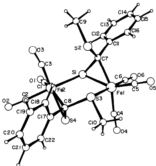
Fig. 2. The structure of compound V, [\text{Fe}(\text{CO})_3\{\text{SC}(\text{Ph})\text{SMe}\}]_2 .
