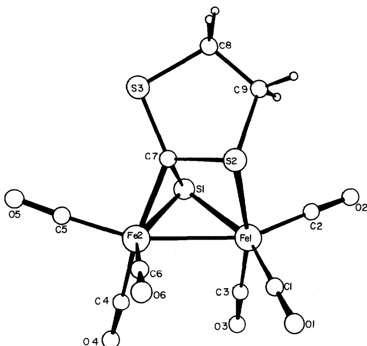
Fig. 1. The structure of compound I, [\text{Fe}_2(\text{CO})_6\{\overline{\text{SCS}(\text{CH}_2)_2\text{S}}\}] .
