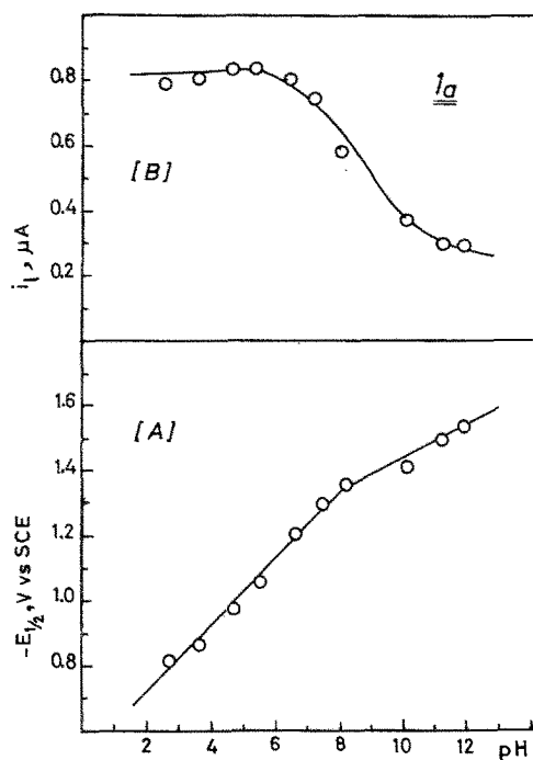
Fig. 3. A: E_{1/2} -, B: i_e - pH plots for the polarographic wave of compound 1a
