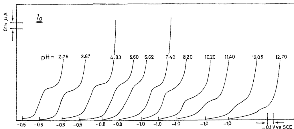
Fig. 2. Polarograms of 10^{-4} \text{ mol dm}^{-3} compound 1a in 50% (v/v) ethanolic Britton-Robinson buffers
