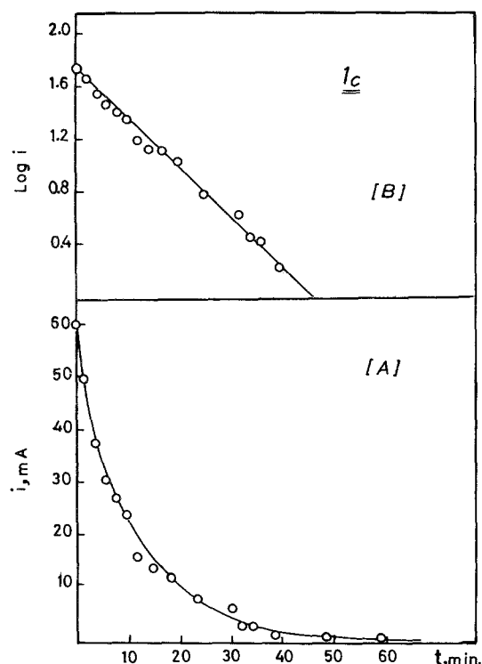
Fig. 1. Controlled potential electrolysis plots of compound 1c ; A: i - t plot., B: \log i - t plot
