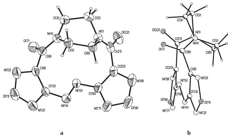
Figure 1. The general view of molecule 7 . Two projections of the molecule, demonstrating conformations of azofurazan and piperazine fragments and their mutual arrangement are shown. Displacement ellipsoids for view a are drawn at the 50% probability level. The view b is represented as a "ball and stick" model for clarity. The bond lengths for azofurazan fragment (Å): C(9)-N(10) 1.301(2), C(9)-C(13) 1.423(2), N(10)-O(11) 1.391(2), O(11)-N(12) 1.358(2), N(12)-C(13) 1.308(2), C(13)-N(14) 1.407(2), N(14)-N(15) 1.244(2), N(15)-C(16) 1.409(2), C(16)-N(17) 1.299(2), C(16)-C(20) 1.425(2), N(17)-O(18) 1.367(2), O(18)-N(19) 1.395(2), N(19)-C(20) 1.296(2).
