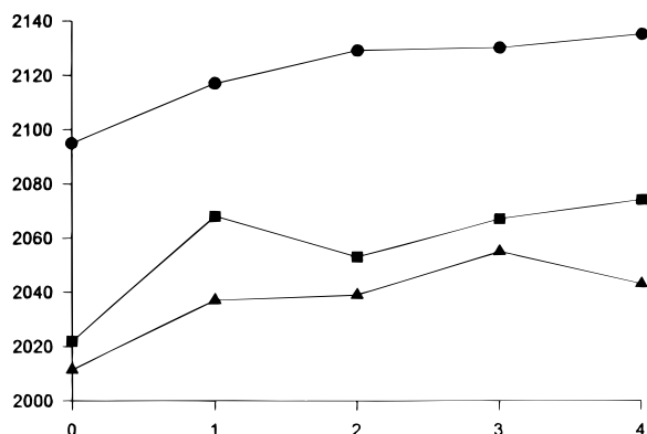
Figure 4. Frequencies of the carbonyl stretching absorptions in \text{Fe}(\text{CO})_4(\text{C}_2\text{H}_{4-x}\text{F}_x) are plotted versus X . The spectra of \text{Fe}(\text{CO})_4(\text{C}_2\text{H}_4) were obtained in the gas phase, and the positions indicated for the low-frequency A_1 and B_1 absorptions of \text{Fe}(\text{CO})_4(\text{C}_2\text{H}_4) are the average of the positions reported in refs 6 and 21. The absorptions reported in light petroleum have been shifted by +10\text{ cm}^{-1} to facilitate comparison with gas-phase absorptions. Symbols: ●, high-frequency A_1 absorption; ■, low frequency A_1 absorption; ▲, B_1 absorption.
