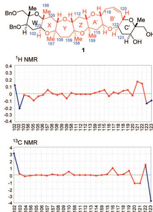
Figure 1. Differences in proton (500 MHz, 1:1 C 5 D 5 N/CD 3 OD) and carbon (125 MHz, 1:1 C 5 D 5 N/CD 3 OD) NMR chemical shifts between MTX and the WXYZA'B'C' ring system ( 1 ). The x- and y-axes represent carbon number and \Delta\delta ( \Delta\delta = \delta_{\text{MTX}} - \delta_{\text{synthetic 1}} in ppm), respectively.
