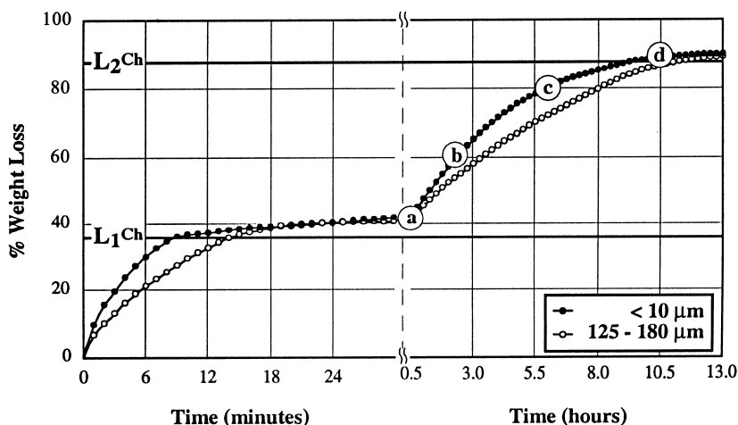
Fig. 3. Isothermal oxychlorination with \text{Cl}_2 + \text{O}_2 of two grain sizes of chromite at 1050°C.
