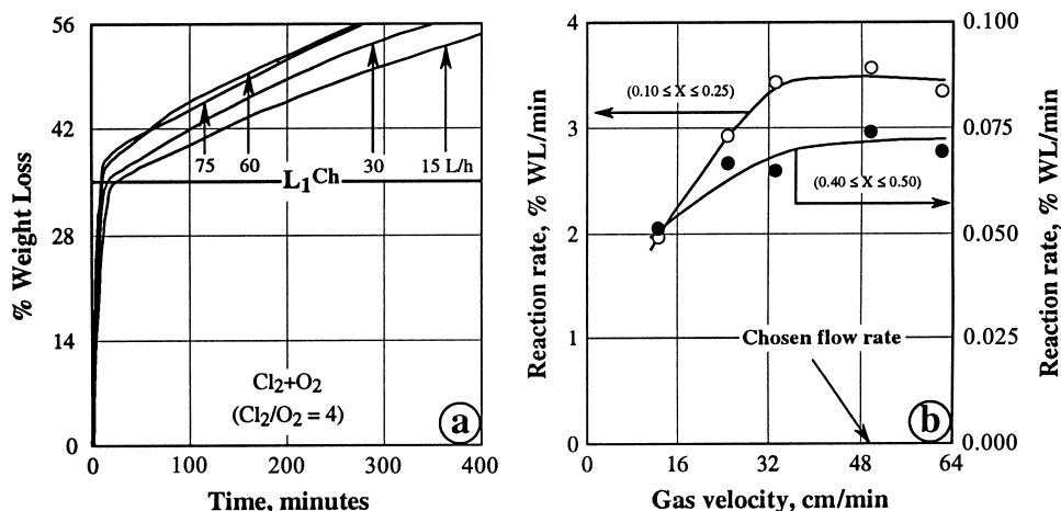
Fig. 5. Isotherms of the chromite oxychlorination using: (a) different gas flow rate; (b) its effect on the reaction rate.
