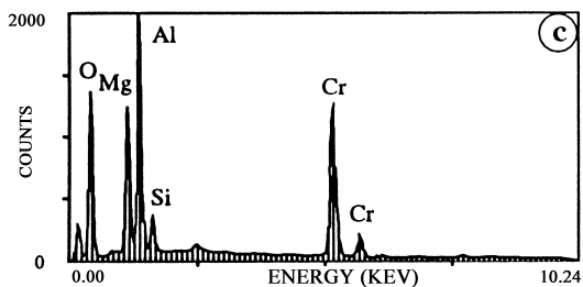
Fig. 4. SEM results of oxychlorination residues of chromite at 1050°C for different reaction extents.
