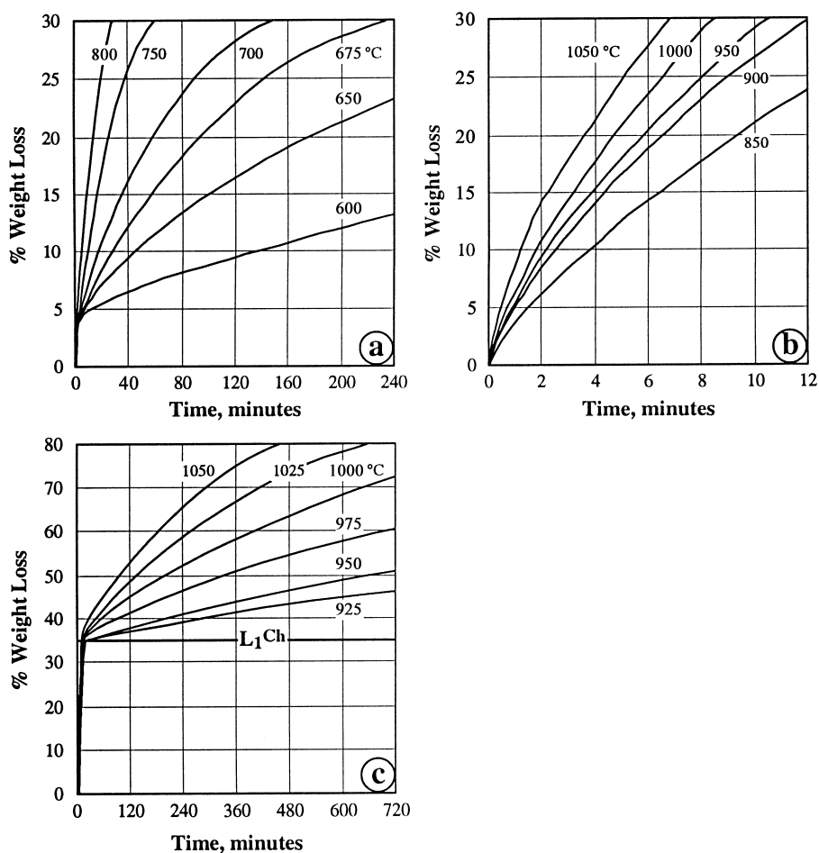
Fig. 6. Isotherms of the chromite oxychlorination with Cl_2 + O_2 between: (a) 600 and 800 °C ( X \leq 0.30 ); (b) 850 and 1050 °C ( X \leq 0.30 ); (c) 925 and 1050 °C ( X \leq 0.80 ).
