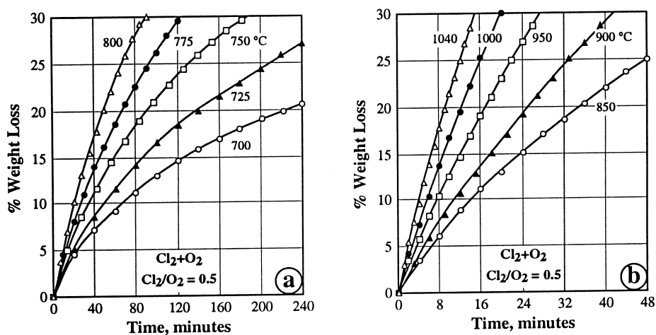
Fig. 10. Isotherms of the chromite oxychlorination with \text{Cl}_2 + \text{O}_2 having a \text{Cl}_2/\text{O}_2 molar ratio equal to 0.5 for: (a) T \leq 800^\circ\text{C} ; (b) T \geq 850^\circ\text{C} .
