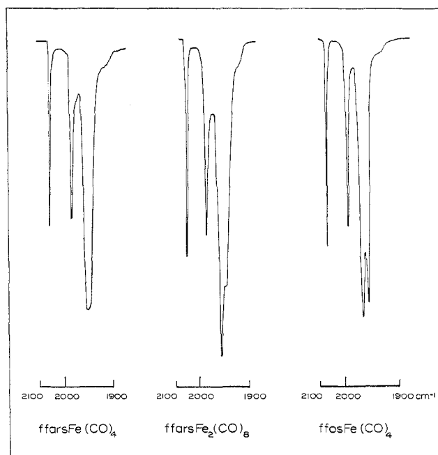
Figure 3.—CO stretching band patterns of \text{Fe}(\text{CO})_4 derivatives (cyclohexane solution).
