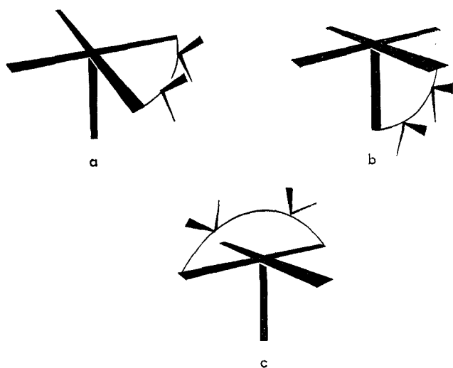
Figure 2.—Possible structures for (chelate) \text{Fe}(\text{CO})_3 complexes based on a square pyramid.
