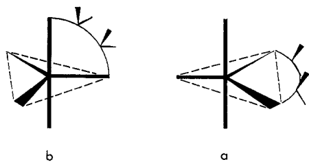
Figure 1.—Possible structures for (chelate)Fe(CO) 5 complexes based on a trigonal bipyramid.
