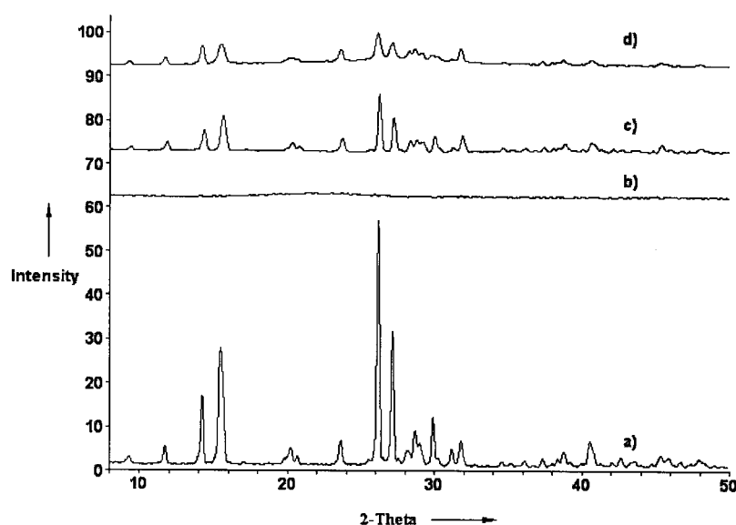
Figure 3. PXRD patterns for a) a single-phase polycrystalline sample of 3 ; b) above sample after heated to 230 °C, at which point all four water molecules are dissociated and the sample color changed from beige to violet; c) sample in b) after placed in water for 30 minutes (the color turned back to beige); and d) sample after repeating the above procedure a)–c) five times.
