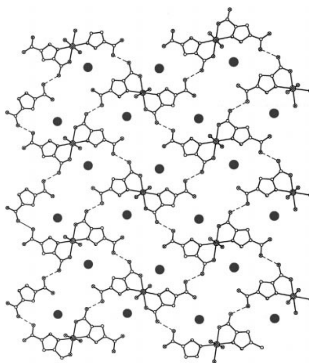
Figure 1. View of the basket-weave-like, two-dimensional hydrogen-bonded network of [\text{M}(\text{H}_2\text{pdc})_2(\text{H}_2\text{O})_2] \cdot 2\text{H}_2\text{O} , \text{M} = \text{Mn} ( 1 ), Fe ( 2 ), Co ( 3 ), Ni ( 4 ), and Zn ( 5 ) along the c axis. Large cross-shaded circles are metal atoms, small cross-shaded, open, and partially shaded circles are O, C, and N atoms, respectively. Large solid circles represent the two solvated water molecules. Hydrogen bonds are indicated by dotted lines.
