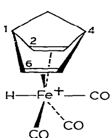
(XXVII)( \text{BF}_4^- )
