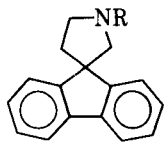
IXa: R = 4-CH 3 C 6 H 4
