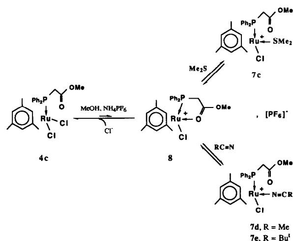
Scheme 3. Reversible coordination of L at the (mesitylene)Ru II centre.
