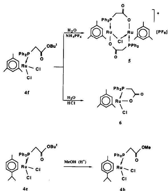
Scheme 1. Reactivity of the tert-butylidiphenylphosphinoacetate derivatives 4f and 4e .
