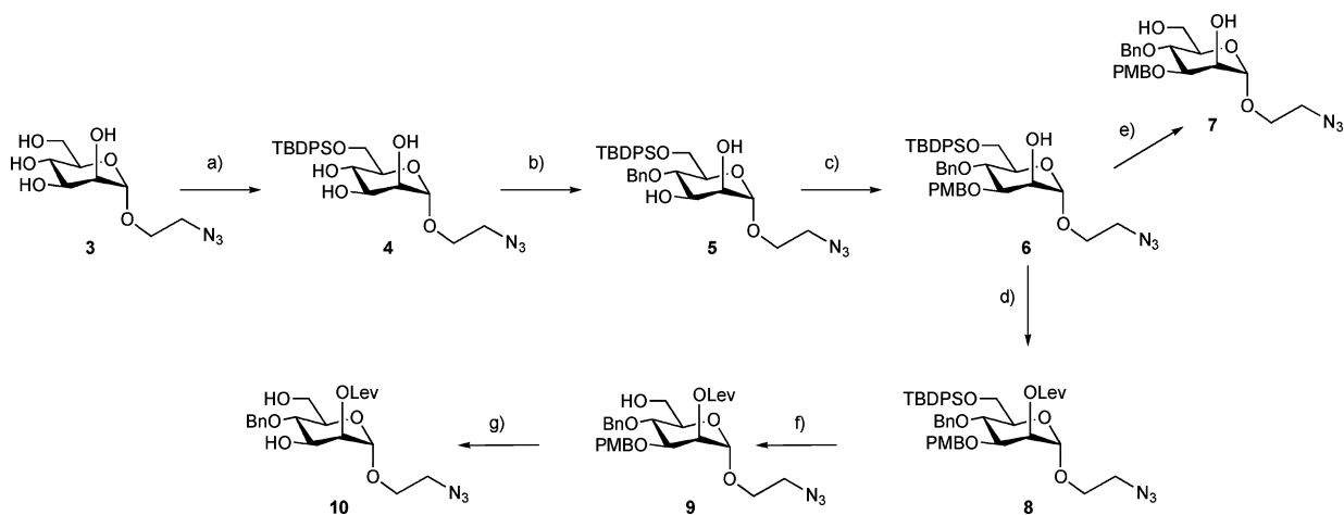
Scheme 1 Synthesis of orthogonally protected mannose derivative 8 and selective deprotections. Reagents and conditions: a) TBDPSCl, Im, DMF, rt, 79%; b) 2,2'-dimethoxypropane, PPTS, acetone; then, BnCl, NaH, DMF, 0 °C to rt; then, TFA, DCM, rt 63% over 3 steps; c) Bu 3 SnO, Tol, Δ; then, PMBCl, Bu 4 NI, Δ, 82%; d) DCC, LevOH, DCM, rt, 88%; e) TBAF, THF, rt, 95%; f) AcOH, THF, 0 °C to rt, then, TBAF, 100%; g) TFA, DCM, -20 °C, 97%.
