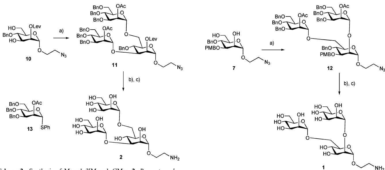
Scheme 2 Synthesis of Manα1-3[Manα1-6]Man 2 . Reagents and conditions: a) 13 (2 equiv.), 4 Å MS, NIS, TfOH, -20 °C, DCM, 78%; b) NaOMe, MeOH, rt; c) H 2 , Pd-C, MeOH, rt, 100%.
