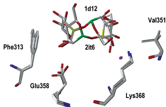
Fig. 6 Superimposition of DC-SIGN/Man \alpha 1-2Man (1d12) complex obtained from the theoretical docking calculation and from the 3D structure of disaccharides (pdb code 2it6). Only the binding pocket with the representative residues is represented here.
