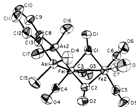
Figure 1. The molecular structure of (diars) \text{Fe}_2(\text{CO})_7 , with the atom numbering scheme shown. Each atom is represented by its ellipsoid of thermal vibration, scaled to enclose 40% of the electron density.
