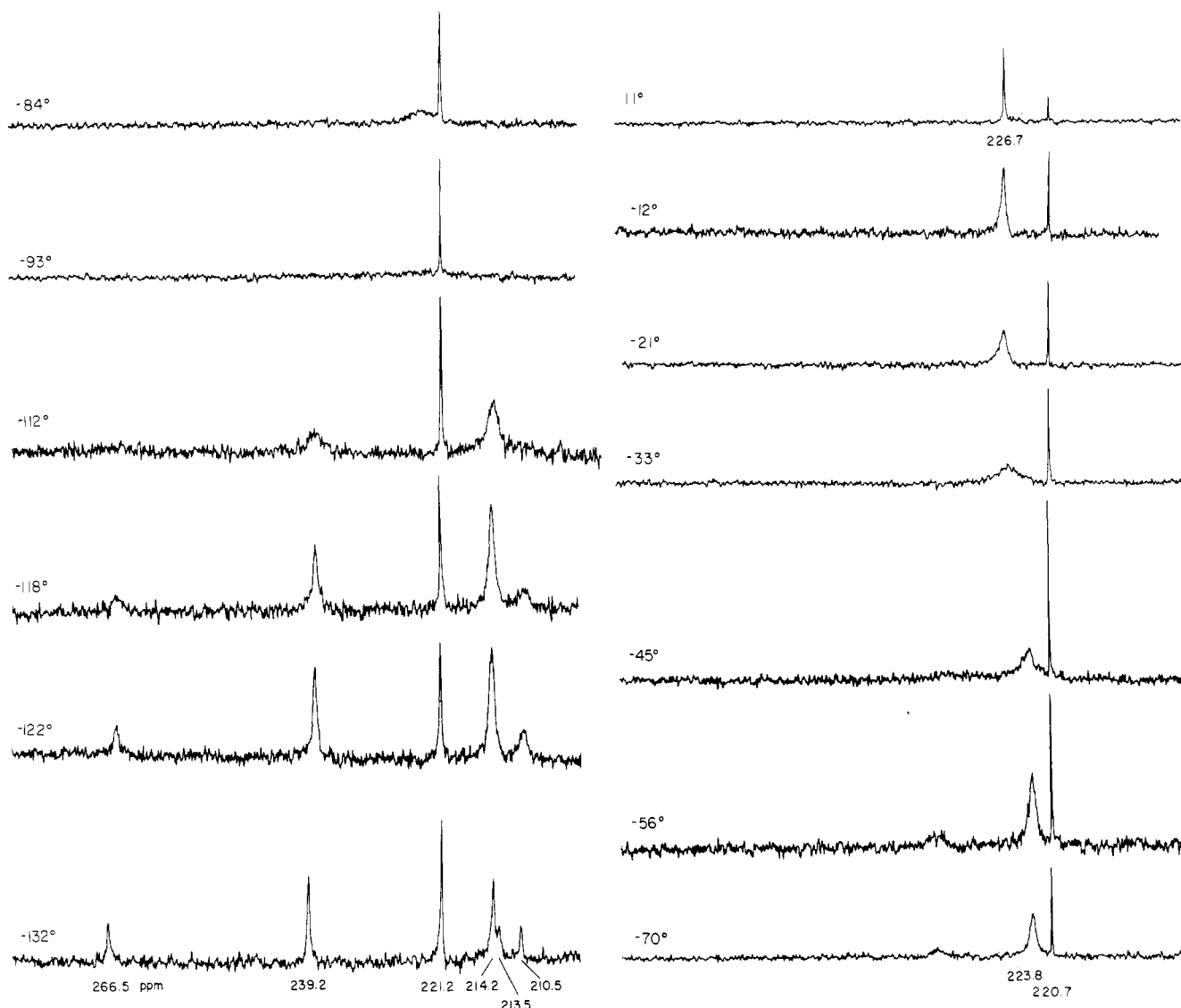
Figure 2. Carbon-13 NMR spectra of (\text{diars})\text{Fe}_2(\text{CO})_7 from -132 to 11^\circ\text{C} . The indicated chemical shifts, in ppm, are downfield from (\text{CH}_3)_4\text{Si} .
