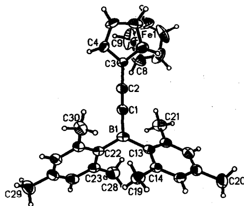
Fig. 4. Molecular structure of ( \eta -C 5 H 5 )Fe( \eta -C 5 H 4 )C≡CB(mes) 2 ( 5b ).
