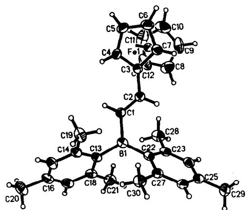
Fig. 2. Molecular structure of (E) -( \eta -C 5 H 5 )Fe( \eta -C 5 H 4 )CH=CHB(mes) 2 ( 3b ).
