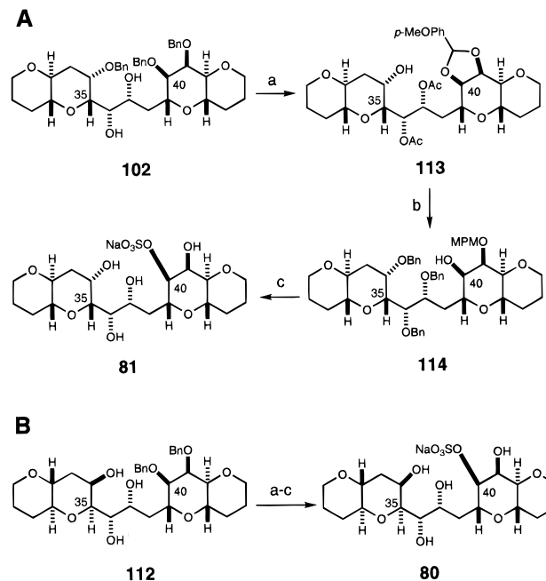
Scheme 16 a
