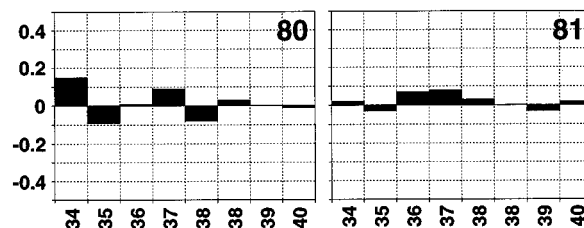
Chart 9. Difference in Proton (500 MHz, 1:1 C 5 D 5 N–CD 3 OD) and Carbon (125 MHz, 1:1 C 5 D 5 N–CD 3 OD) Chemical Shifts between MTX and Each of 80 and 81
