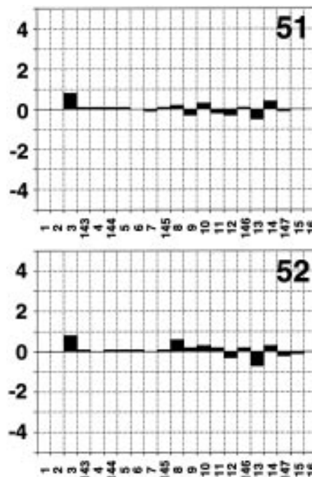
Chart 6. Difference in Carbon Chemical Shifts between MTX and Each of 51 and 52 (125 MHz, 1:1 C 5 D 5 N-CD 3 OD)
