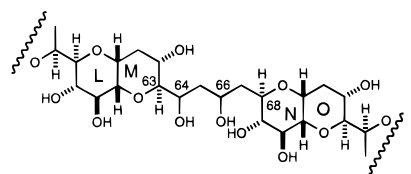
C.63-C.68 partial structure of MTX
