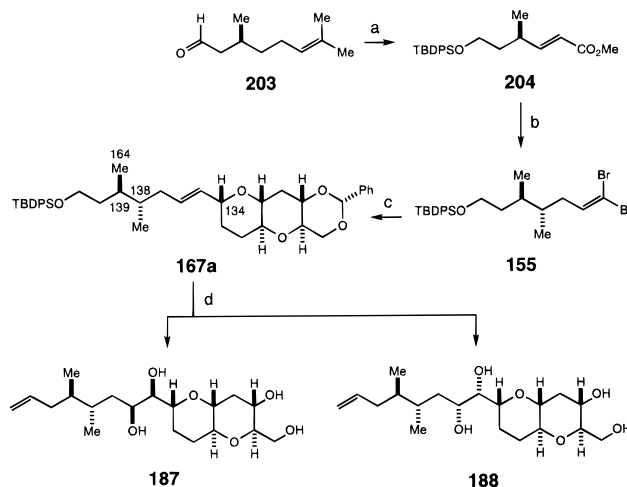
Scheme 31 a
