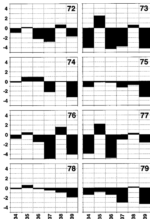
Chart 8. Difference in Carbon Chemical Shifts between MTX and Each of 72–79 (125 MHz, 1:1 C 5 D 5 N–CD 3 OD)
