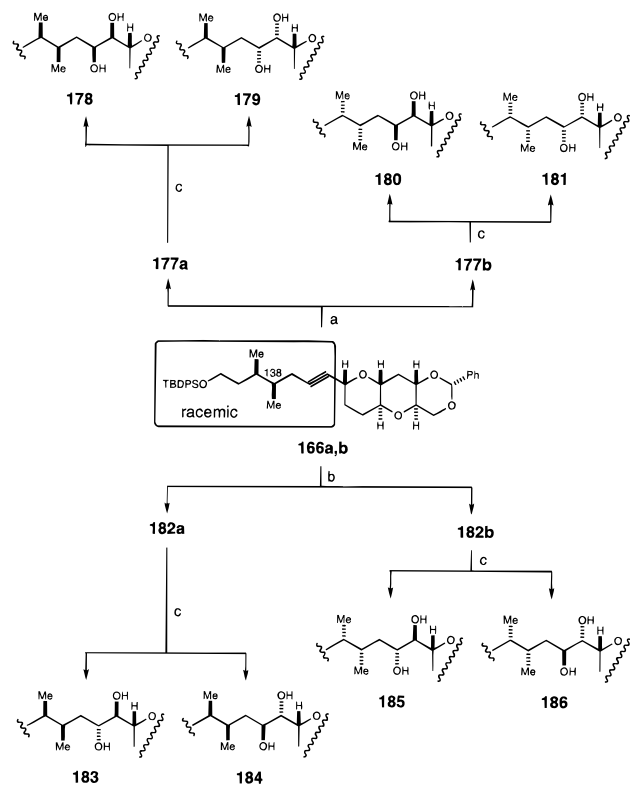
Scheme 29 a
