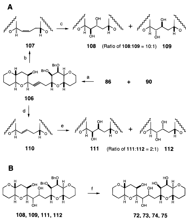
Scheme 15 a
