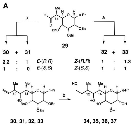
Scheme 5 a
