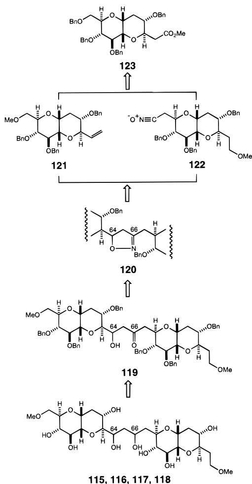
Scheme 17
