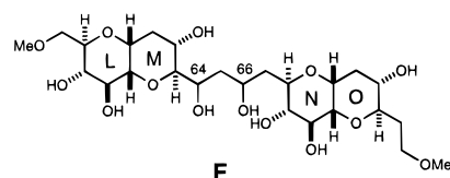
C.63-C.68 partial structure of MTX
