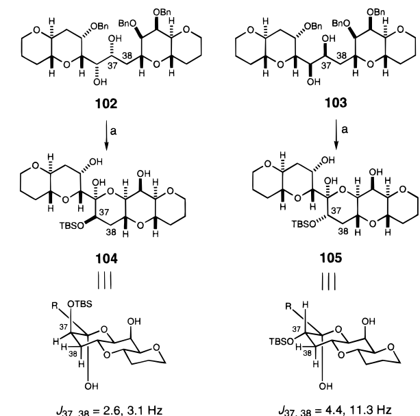
Scheme 14 a
