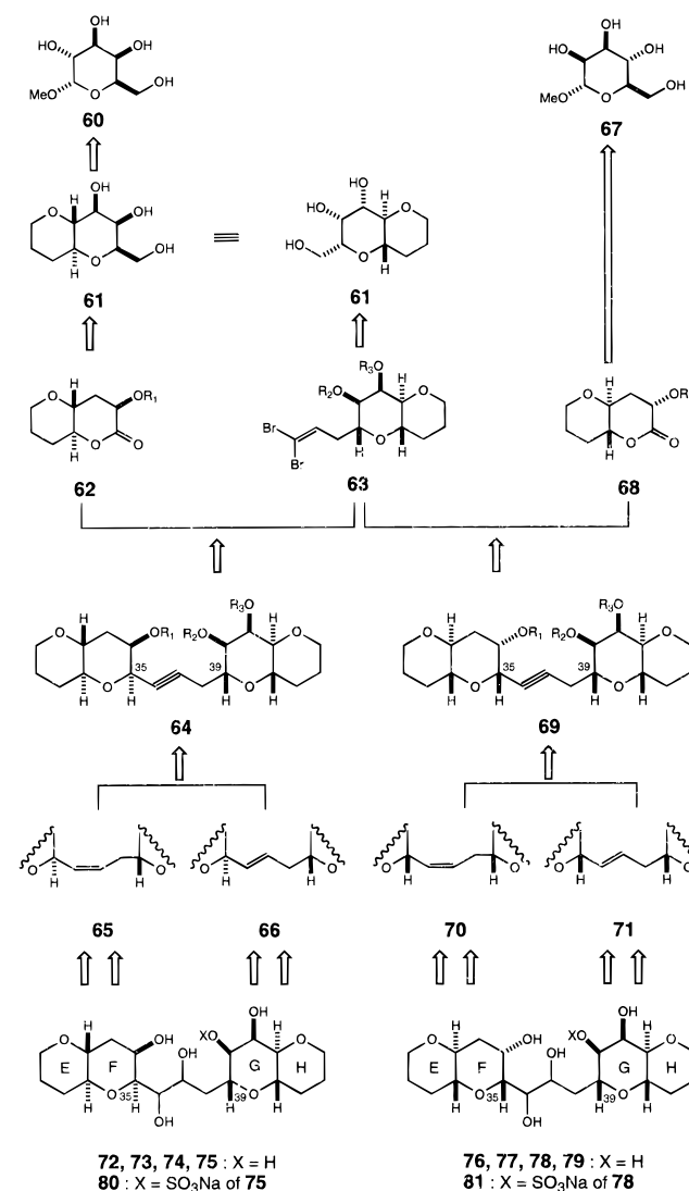
Scheme 9
