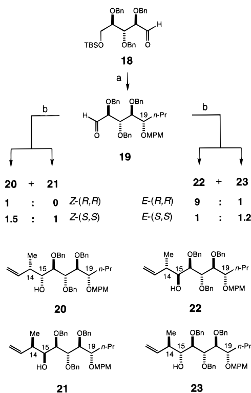
Scheme 3 a
