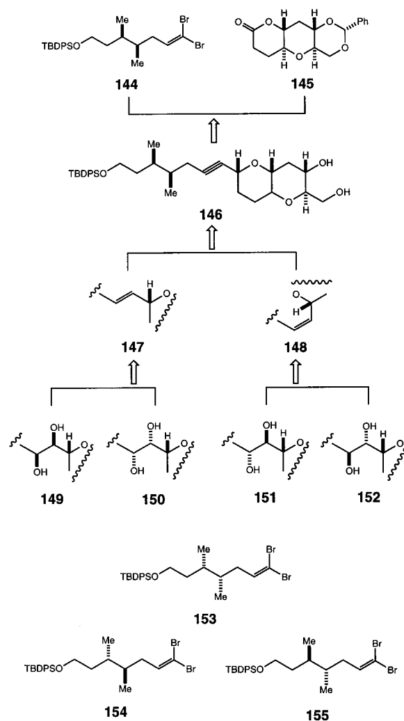
Scheme 24
