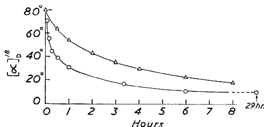
FIG. 1. Mutarotation of 6-deoxy-6-fluoro-2,3,4-tri- O -methyl-D-galactono-1,5-lactone (o) and 2,3,4-tri- O -methyl-D-galactono-1,5-lactone (Δ) (c 0.36 in water).
