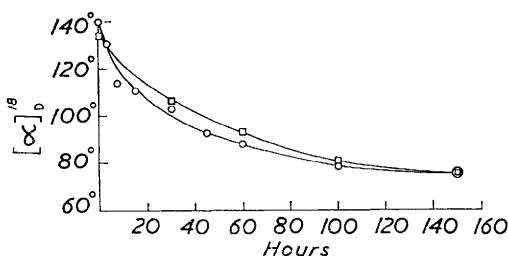
FIG. 2. Mutarotation of 6-deoxy-6-fluoro- \alpha -D-galactose (○) and \alpha -D-galactose (□) (c 0.4 in water).
