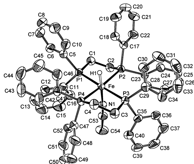
Fig. 1. ORTEP drawing [24] of the cationic part of 2b , [FeH(NCCH_3)(dppe)_2]^+ , showing the atom-labeling scheme and 50% probability thermal ellipsoids.
