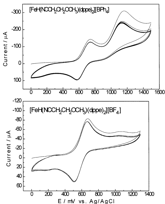
Fig. 4. Cyclic voltammograms (300 mV/s) in 0.1 M [\text{nBu}_4\text{N}][\text{BF}_4] - \text{CH}_2\text{Cl}_2 solutions of 3b (top) and 3c (bottom).
