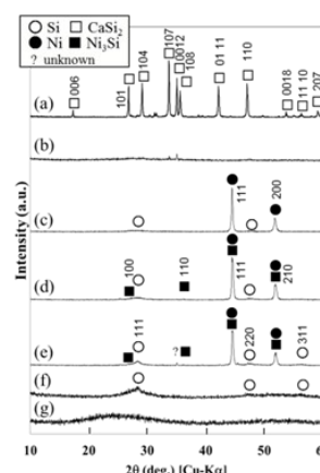
Figure 1. Powder XRD patterns for (a) \text{CaSi}_2 (raw material), (b) Ca-siloxene, synthesized (c) S-300, (d) 400 and (e) 500 samples, and (f) commercial Si and (g) \text{SiO} .
