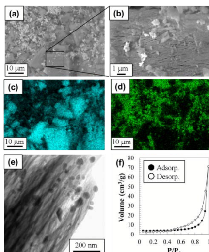
Figure 2. (a,b) SEM images, SEM-EDX elemental mapping image for (c) Si and (d) Ni, (e) STEM image and (f) N_2 adsorption isotherm for the synthesized S-400 sample.
