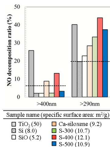
Figure 4. Nitrogen monoxide decomposition ratio over reference samples ( \text{TiO}_2 , Si, SiO, Ca-siloxene) and synthesized samples (S-300, 400 and 500). The dotted lines indicate the blank data (ratio observed without a catalyst).
