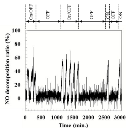
Figure 5. Nitrogen monoxide decomposition rate as a function of the light ( >290 \text{ nm} ) irradiation time for the synthesized sample S-400.
