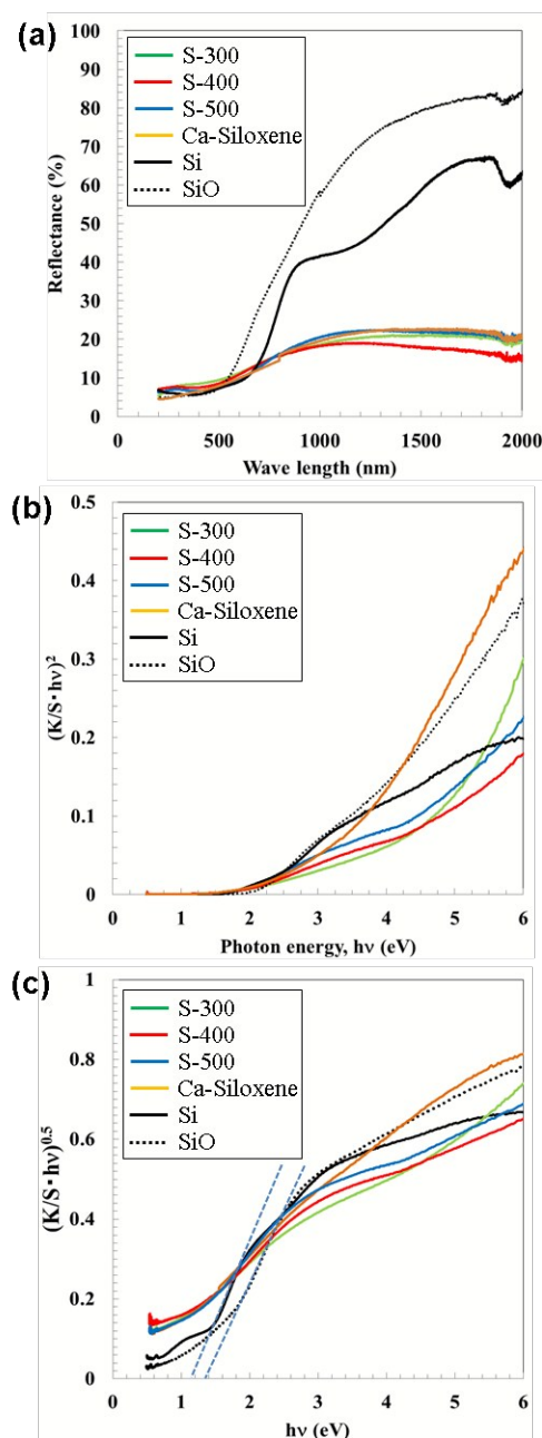
Figure 3. (a) Diffuse reflectance spectra, and (b,c) Tauc plots of Kubelka-Munk absorption (K/S) as a function of photon energy ( h\nu ) under the assumption of (b) direct and (c) indirect transition for reference samples (Si, SiO , Ca-siloxene) and synthesized samples (S-300, 400 and 500).
