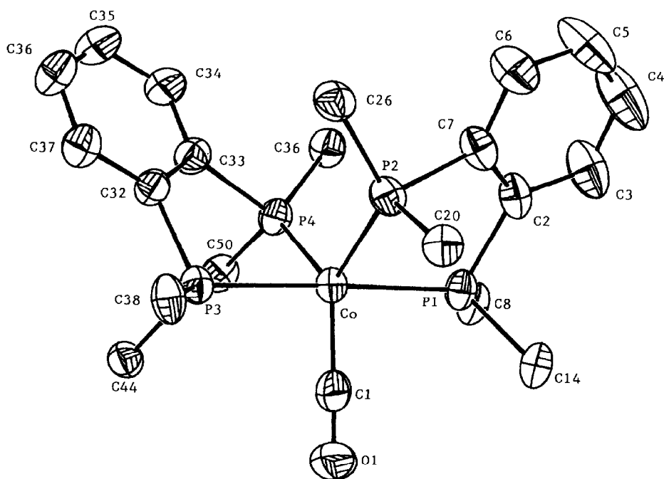
Fig. 1. ORTEP drawing of \text{Co(CO)(}o\text{-C}_6\text{H}_4[\text{PPh}_2]_2)^+ . Eight phenyl groups are represented only by their ipso carbon atoms for clarity. The ellipsoids are drawn to 30% probability boundaries.
