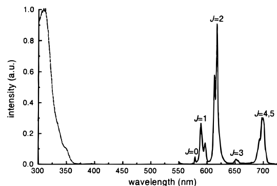
Figure 2. Excitation spectrum (dashed line, \lambda_{\text{em}} = 615 nm) and emission spectrum ( \lambda_{\text{ex}} = 310 nm) of a 10^{-4} M solution of (Eu)1 in methanol. The emission bands correspond to ^5\text{D}_0 \rightarrow ^7\text{F}_j transitions and were recorded with a 1 nm emission bandwidth.
