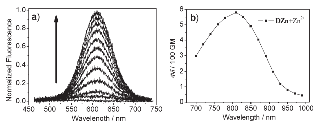
Figure 1. (a) TP emission spectra of 1 \mu\text{M} DZn (MOPS buffer) in the presence of free \text{Zn}^{2+} (0–6 \mu\text{M} ). (b) TP action spectra of 1 \mu\text{M} DZn in the presence of 6 \mu\text{M} free \text{Zn}^{2+} .
