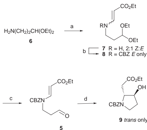
Scheme 3 Reagents and conditions: (a) \text{HC}\equiv\text{CCO}_2\text{Et} , \text{Et}_2\text{O} , rt, 3 days, 100% crude; (b) n\text{-BuLi} , THF, -78^\circ\text{C} , 30 min, then \text{CBZCl} , warm to rt, 45 min, 100% crude; (c) \text{TsOH}\cdot\text{py} , \text{H}_2\text{O} , \text{Me}_2\text{CO} , reflux, 7 h, 30%; (d) \text{SmI}_2 , THF, HMPA, \text{MeOH} , 0^\circ\text{C} , 90 min, 53%.
