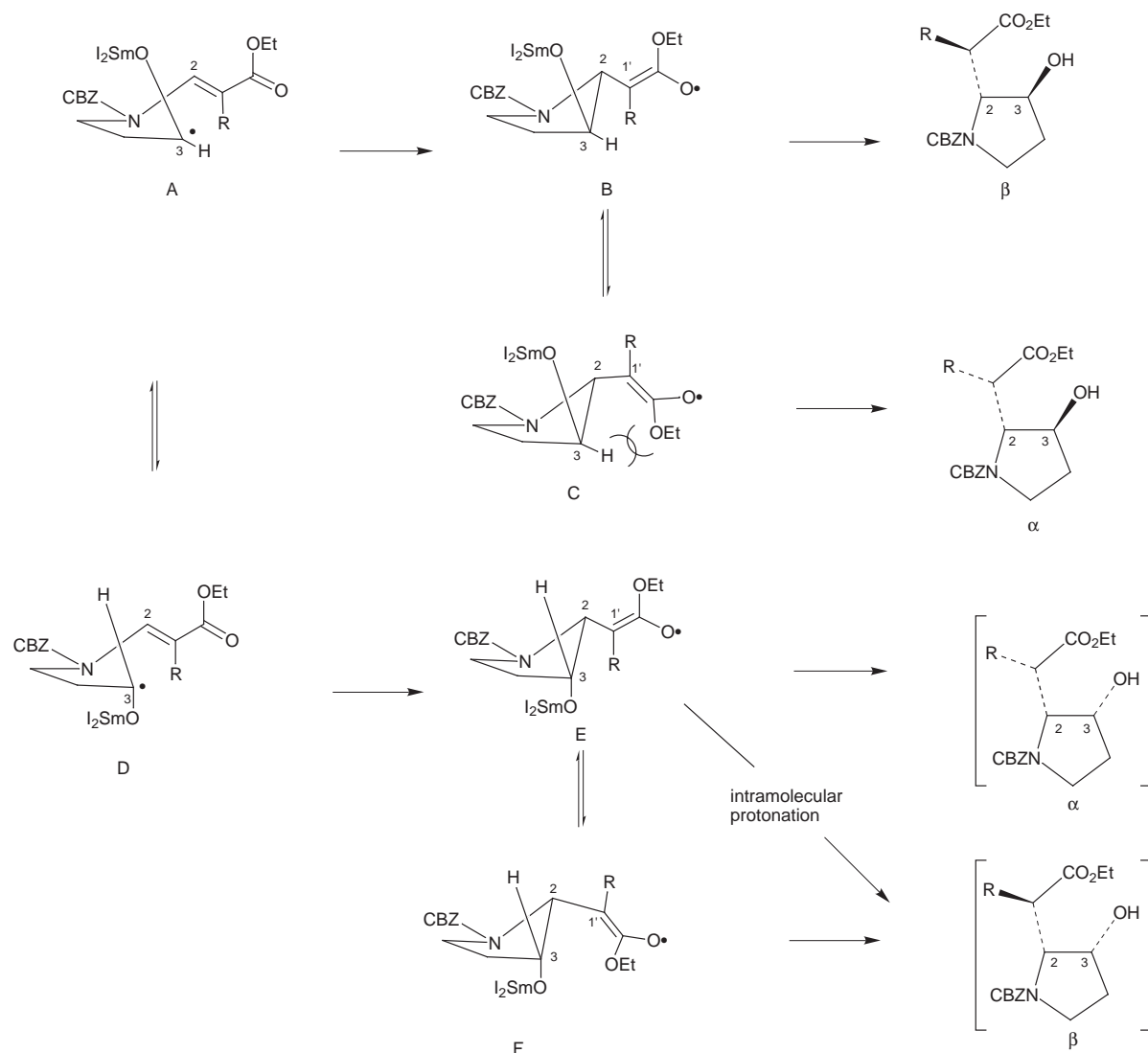
Fig. 1 Possible transition states for the 5- exo-trig cyclisations of 4 and 5 . Unless shown otherwise protonation of B, C, E and F is assumed to occur from the most open ( exo ) face (from the back face as drawn). The cis -products from E and F are shown as hydroxy esters, although in fact only the cis -lactone 16 was isolated.
