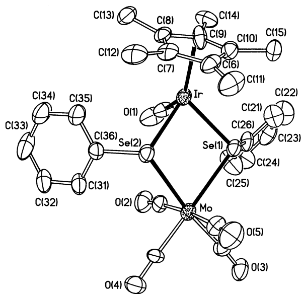
Fig. 1. Molecular structure of Cp*Ir(CO)(μ-SePh) 2 [Mo(CO) 4 ] ( 10b )
