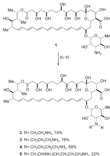
Scheme 1. a) FmocNH(CH 2 ) n CHO ( n = 1–3) or FmocNH 2 (CH 2 ) 4 -(NHfmoc)CHCH 2 CHO, NaBH 3 CN, DMF; b) piperidine, DMSO.
