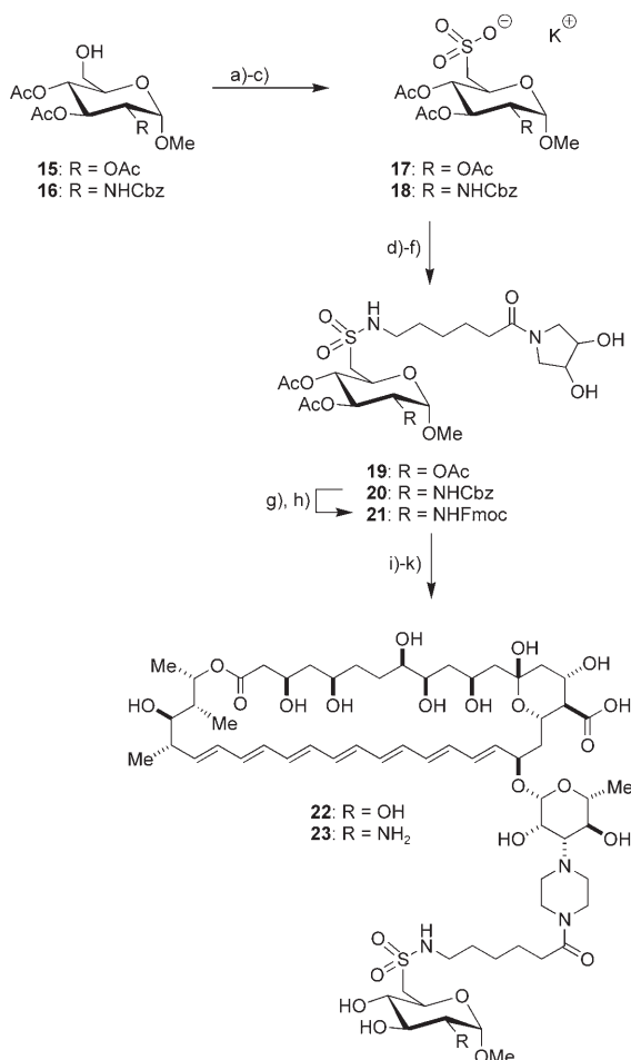
Scheme 4. a) MsCl, Et 3 N, CH 2 Cl 2 ; b) KSAc, DMF; c) H 2 O 2 , KOAc, AcOH, 79% for 17 , 60% for 18 over three steps; d) SO 2 Cl 2 , PPh 3 , CH 2 Cl 2 ; e) Et 3 N, 24 ; f) K 2 OsO 4 , NMO, acetone/H 2 O/ t BuOH, 24% for 19 , 46% for 20 over three steps; g) H 2 , Pd/C; h) FmocSuc, Na 2 CO 3 , H 2 O/dioxane 26% over two steps; i) NaIO 4 , SiO 2 , H 2 O/CHCl 3 ; j) AmB, NaBH 3 CN, DMF; k) K 2 CO 3 , piperidine, H 2 O/MeOH, 59% for 22 , 66% for 23 over three steps.
