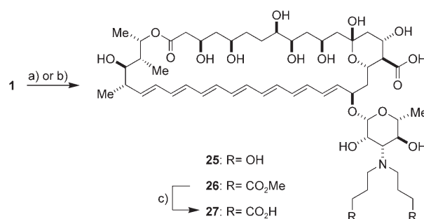
Scheme 5. a) i) TBSOCH 2 CH 2 CHO, NaBH 3 CN, DMF, ii) HF/pyridine, 28% for 25 ; b) MeO 2 CCH 2 CH 2 CHO, NaBH 3 CN, DMF, 45% for 26 ; c) LiOH, THF/H 2 O, 43%.
