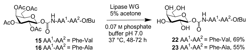
Scheme 4. Initial enzymatic cleavage of acetyl groups.
