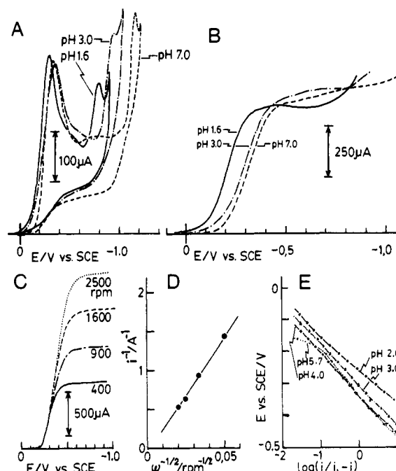
Figure 5. (A) CV curves for oxygen reduction at Co II CRPc/HOPG (scan rate 100 mV/s). (B) RDE responses for oxygen reduction at Co II CRPc/HOPG at various pH values (scan rate 10 mV/s). (C) RDE responses for oxygen reduction at Co II CRPc/HOPG at various rotation speeds (pH 13, scan rate 10 mV/s). (D) Koutecky-Levich plots constructed from the plateau current in (D). (E) Tafel type plots from RDE data at Co II CRPc/HOPG for the first oxygen reduction process.
