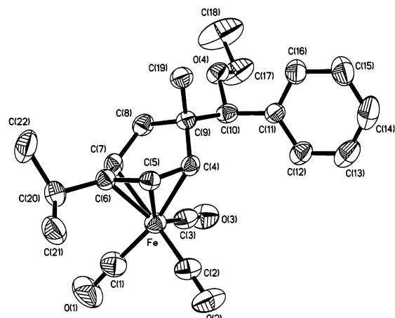
Figure 5. Molecular structure of 23 .
