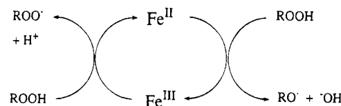
Scheme 1. Key Mechanistic in the Catalytic Oxidation of Alkanes: Oxidation and Reduction of Alkyl Hydroperoxides by Perhalogenated Iron Porphyrins
