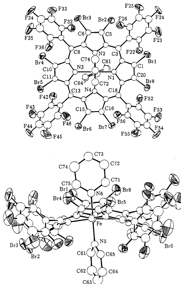
Figure 2. ORTEP diagrams of \text{Fe}^{\text{II}}(\text{TFPPBr}_8)(\text{py})_2 with ellipsoids drawn at the 50% probability level.
