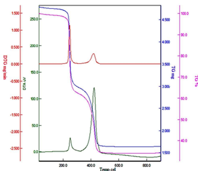
Figure 4. TGA curve of Cu(II) immobilized on \text{Fe}_3\text{O}_4@\text{SiO}_2@\text{L-Arginine} .
