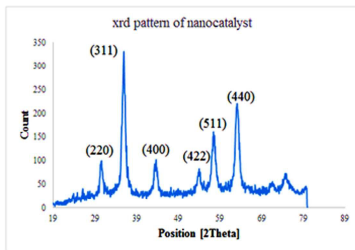
Figure 3. The X-ray diffraction pattern of Cu(II) immobilized on \text{Fe}_3\text{O}_4@\text{SiO}_2@\text{L-Arginine} nanoparticle.
