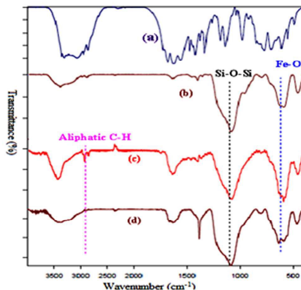
Figure 1. FT-IR spectra of pure L-Arginine (a), \text{Fe}_3\text{O}_4@\text{SiO}_2 (b) \text{Fe}_3\text{O}_4@\text{SiO}_2@\text{L-Arginine} (c) and Cu(II) immobilized on \text{Fe}_3\text{O}_4@\text{SiO}_2@\text{L-Arginine} (d).
