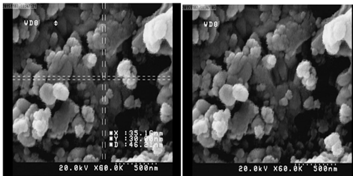
Figure 2. SEM image of Cu(II) immobilized on \text{Fe}_3\text{O}_4@\text{SiO}_2@\text{L-Arginine} .
