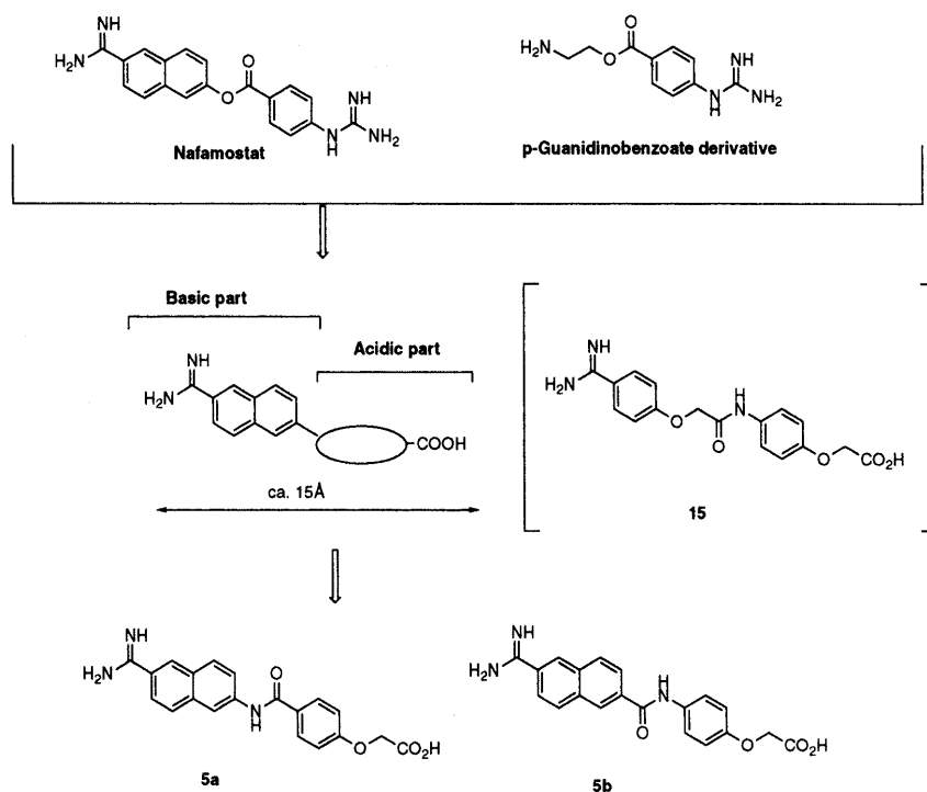
Fig. 1. Design of Active Compounds 5a and 5b Starting from Nafamostat
