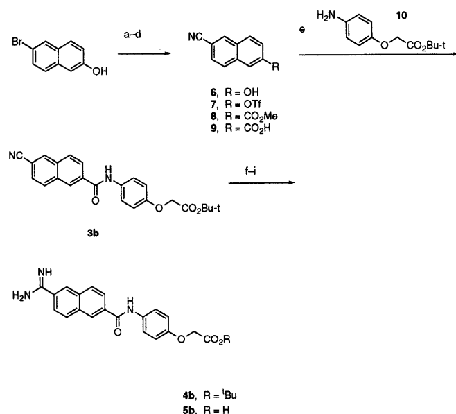
Chart 2. Preparation of 5b
