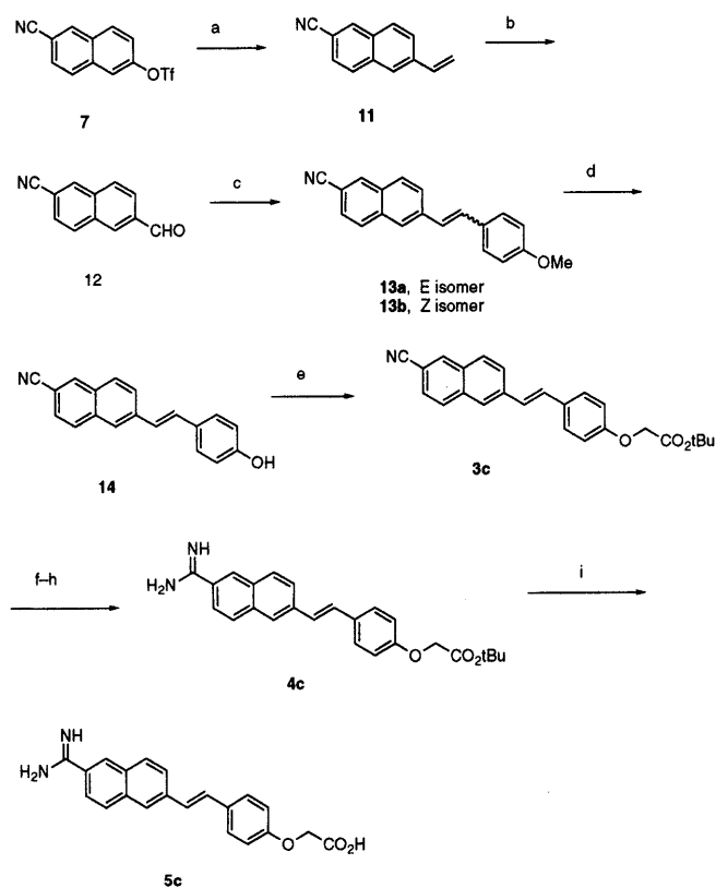
Chart 3. Preparation of 5c
