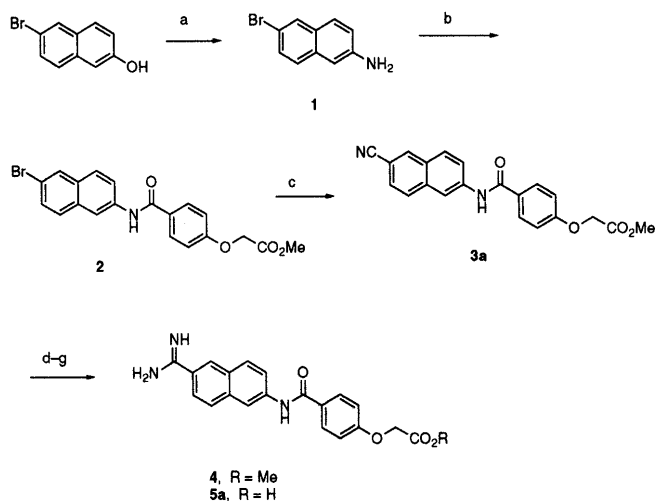
Chart 1. Preparation of 5a
