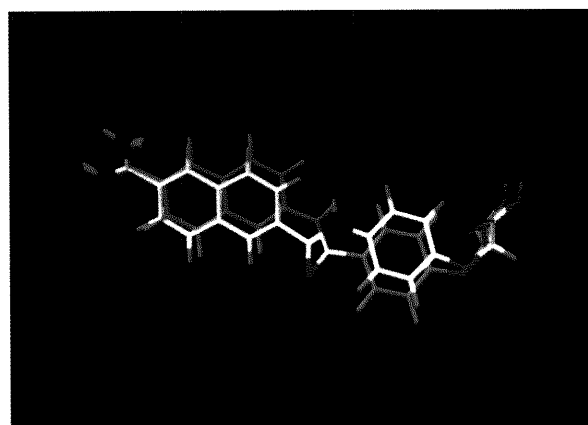
Fig. 8. Superimposition of 5b (White) and 5a (Green)
