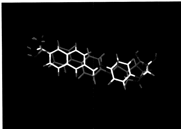
Fig. 3. Superimposition of BIBU-52 (Green) and 5b (White)
