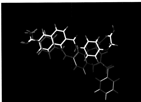
Fig. 4. Superimposition of SB207448 (Green) and 5b (White)
