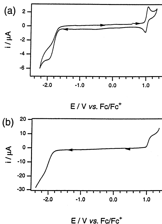
Fig. 10. Cyclic and rotating disc voltammograms of 9b in CH_2Cl_2 at -50^\circ C .
