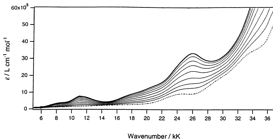
Fig. 11. Electronic spectra recorded during the one-electron oxidation of 9b in \text{CH}_2\text{Cl}_2 at -50^\circ\text{C} . (---) First scan = 9b . (—) Final scan = 9b + .
