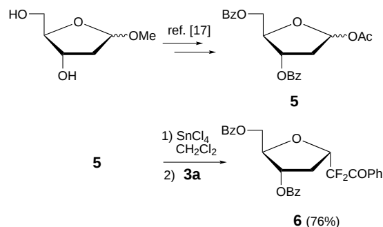
Scheme 5. Reaction of difluoroenoxyisilane 3a with a 2-deoxy glycofuranosyl donor leading to a 2-deoxy difluoro-C-glycoside.
