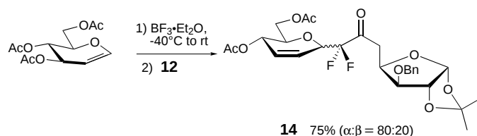
Scheme 9. Application to a carbohydrate derived difluoroenoxyisilane in the D-glucal series.
