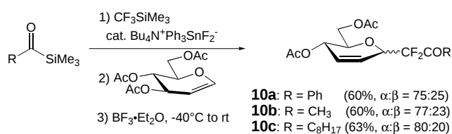
Scheme 7. Reaction of difluoroenoxyisilanes with tri- O -acetyl-D-glucal.
