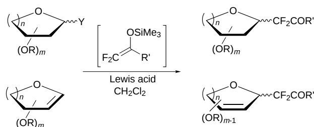
Scheme 3. Application of the methodology to glycosyl donors.
