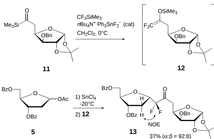
Scheme 8. Application to a carbohydrate derived difluoroenoxyisilane in the 2-deoxy furanose series.
