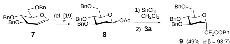
Scheme 6. Reaction of difluoroenoxyisilane 3a with a 2-deoxy pyranosyl donor.
