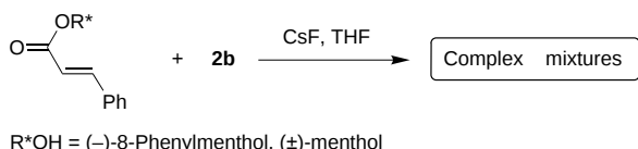
Scheme 5. Reaction of in situ generated azomethine ylides ( 3 ) with cinnamates.
