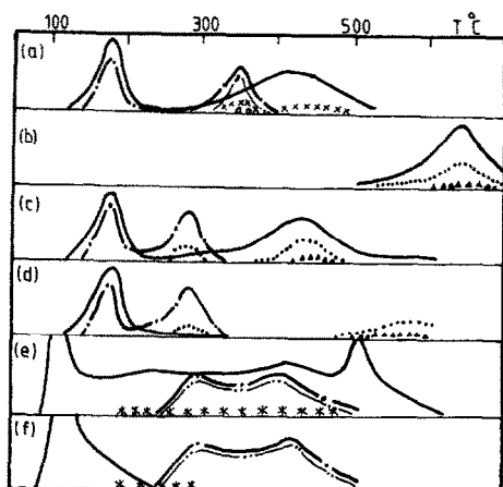
Fig. 2. EG curves of solid state redox reaction of iron oxalate with sodium nitrate and tin chloride. a, Iron(III) oxalate in hydrogen; b, sodium nitrate in hydrogen; c, 1:5 mole iron oxalate and sodium nitrate in hydrogen; d, 1:5 mole iron oxalate and sodium nitrate in helium; e, 1:3 mole iron oxalate with tin chloride in hydrogen; f, 1:3 mole iron oxalate with tin chloride in helium. — \text{H}_2\text{O} ; ..... \text{O}_2 , NO; ▲▲▲ \text{NO}_2 ; -.-.- \text{CO}_2 ; ●—● CO; ××× \text{CH}_4 ; *** HCl; ○○○ \text{C}_2 .
