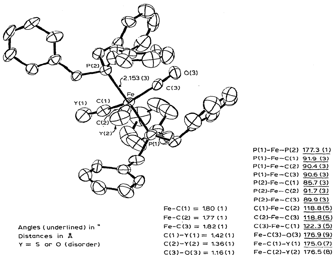
Fig. 1. The structure of [\text{Fe}(\text{CO})_2\{\text{P}(\text{OPh})_3\}_2(\text{CS})] .
