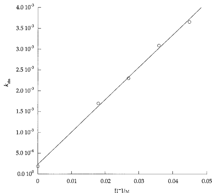
Fig. 5. Plot of k_{\text{obs}} vs. [I^-]
