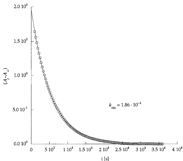
Fig. 3. Decay of the MLCT band in (\text{CyDAB}^H)\text{PtMe}_2 ( 1g ) during reaction with (\text{TMEDA})\text{PtI}_2\text{Me}_2
