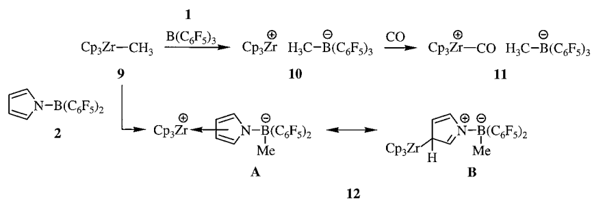
Scheme 2. Reaction of 9 with \text{B}(\text{C}_6\text{F}_5)_3 ( 1 ) and ( N -pyrrolyl) \text{B}(\text{C}_6\text{F}_5)_2 ( 2 ).
