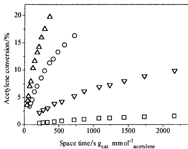
Fig. 2. Conversions of acetylene hydration on Cd-clinoptilolite at 393 K ( \square ), 413 K ( \nabla ), 433 K ( \circ ), and 453 K ( \triangle ) as a function of space-time. The initial partial pressures for acetylene and water are 33 and 67 kPa, respectively.
