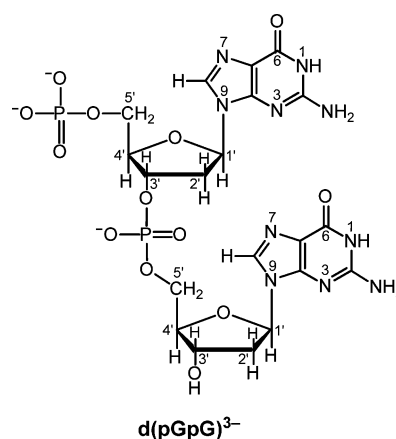
Fig. 1 Chemical structure of the trianion of 2'-deoxyguanylyl(5'→3')-2'-deoxy-5'-guanylic acid, i.e., 2'-deoxyguanylyl(5'→3')-2'-deoxy-5'-guanylate, abbreviated as d(pGpG) 3− , and also known 6 as 2'-deoxy[5'-phosphate-guanylyl-(3'→5')-guanosine]. The two guanosine units are shown in their dominating anti conformation. 14 Note, species written in the text without a charge, e.g., d(pGpG), either do not carry one or represent the species in general (i.e., independent of their protonation degree); which of the two possibilities applies is always clear from the context.
