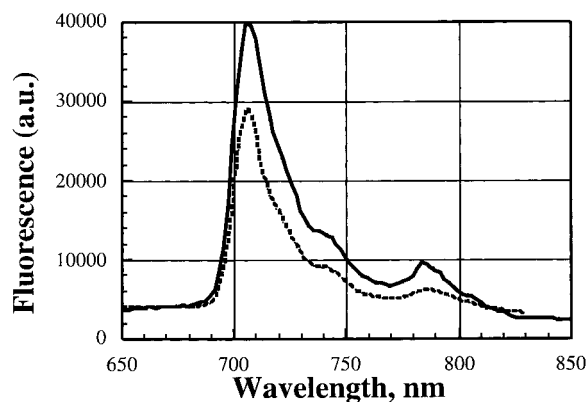
Figure 2. Fluorescence emission spectrum of (a) (—) 1 and (b) (---) 2 in methylcyclohexane at 77 K. (The excitation wavelength was at 400 nm.)
