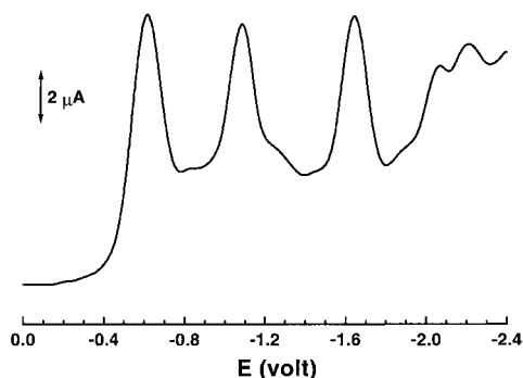
Figure 8. Square-wave voltammogram of 1 in toluene:acetonitrile (3:1 v/v). (Scan rate = 100 mV/s; RE; SCE; WE, glassy carbon; CE, Pt; supporting electrolyte, 0.1 M tetrabutylammonium perchlorate.)
