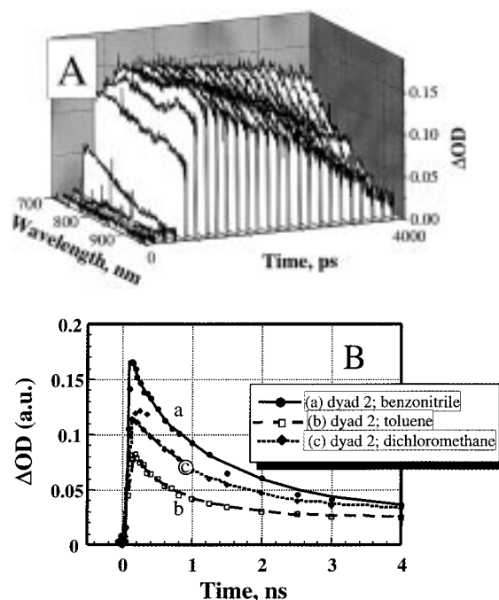
Figure 5. (A) Time-resolved transient absorption spectra showing the decay of singlet and formation of triplet excited states following the 355-nm laser pulse excitation of 2 in toluene. (B) Absorption–time profiles showing the decay of singlet dyad, 2 , in different solvents at monitoring wavelength of 900 nm.
