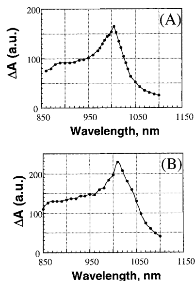
Figure 9. Transient absorption spectrum (near-IR) of (A) 1 and (B) 2 obtained upon pulse radiolysis of 2.0 \times 10^{-5} M of the respective functionalized fullerene derivative in a nitrogen-saturated solvent mixture containing 80 vol % toluene, 10 vol % 2-propanol, and 10 vol % acetone.
