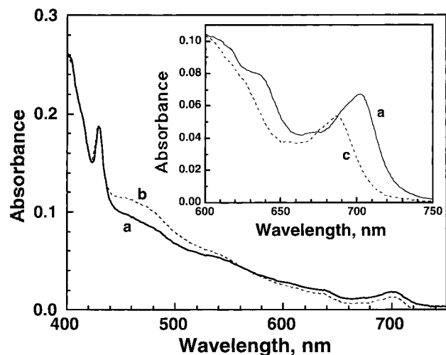
Figure 1. Absorption spectra of dyad 2 (trace a) and model system 1 (trace b), in dichloromethane. Inset shows the changes in the long-wavelength absorption band of dyad 2 in dichloromethane on addition of TFA. The concentrations of TFA were (a) 0 mM and (c) 25 mM.
