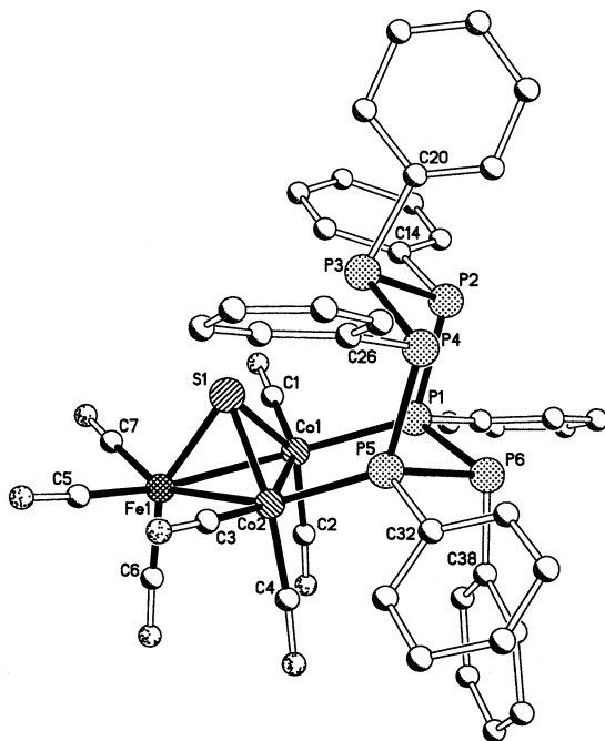
Fig. 2. Molecular structure of [\text{Co}_2\text{Fe}(\mu_3\text{-S})\{\mu\text{-cyclo-(PhP)}_6\}(\text{CO})_7] ( 2 ) including the atom numbering scheme. All hydrogen atoms have been omitted for clarity.
