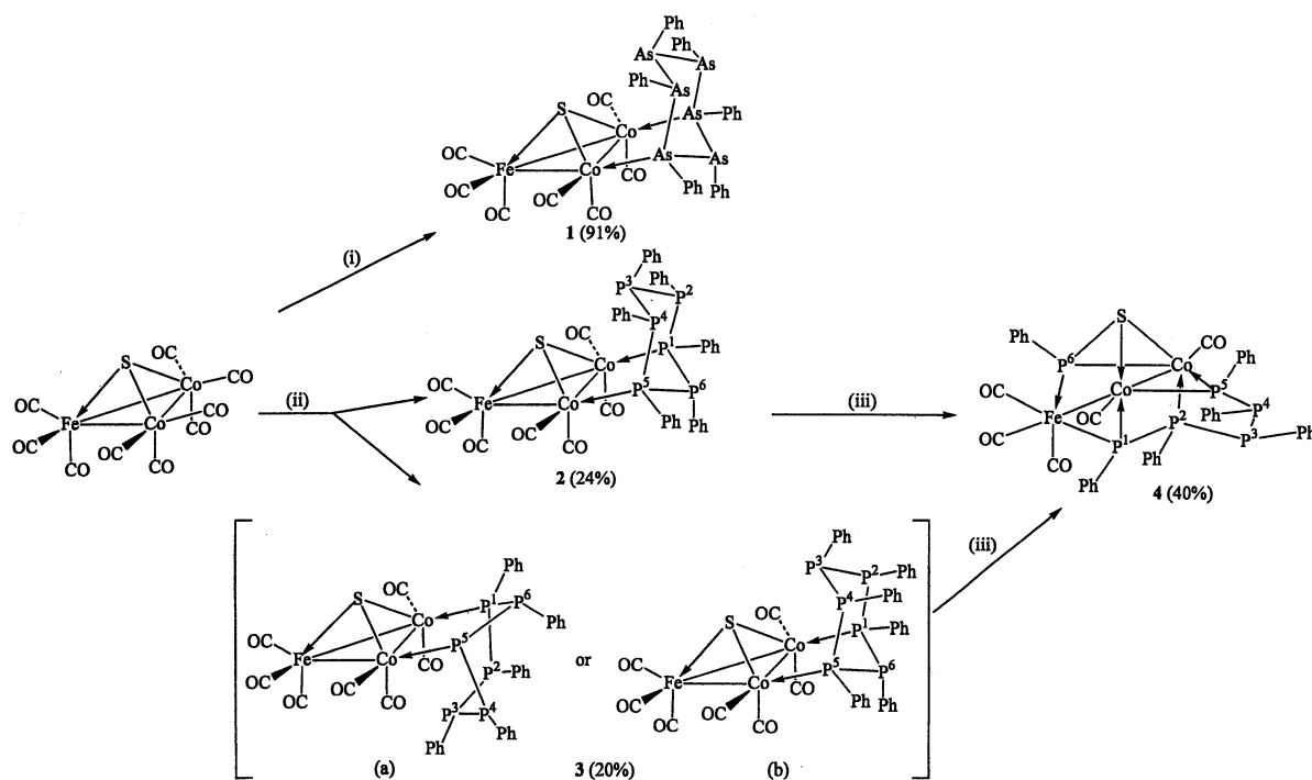
Scheme 1. Reagents and conditions: (i) 70 °C, 22 h, cyclo -(PhAs) 6 , C 7 H 8 ; (ii) 70 °C, 22 h, cyclo -(PhP) 6 , C 7 H 8 ; (iii) 120 °C, 3 h, C 7 H 8 .
