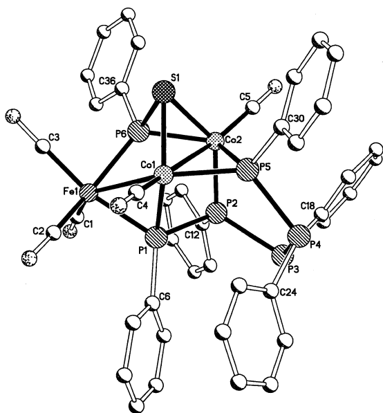
Fig. 3. Molecular structure of [\text{Co}_2\text{Fe}(\mu_3\text{-SPPPh})(\mu\text{-}\eta^2\text{:}\eta^2\text{:}\eta^1\text{-P}_5\text{Ph}_5)(\text{CO})_5] ( 4 ) including the atom numbering scheme. All hydrogen atoms have been omitted for clarity.
