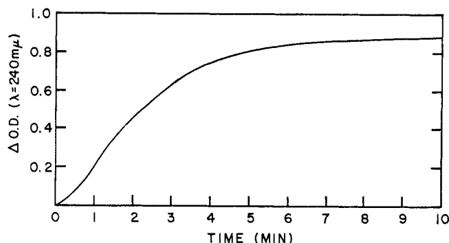
Figure 4. Change of optical density at 240 mμ during the reaction of \beta -benzyl-N-carbobenzyloxy-L-aspartyl-(O-acetyl)-DL-serine methyl ester (I) ( 3.2 \times 10^{-4} M , 1-cm path) in dioxane-water (1:2 v/v), phosphate buffer, pH 10.9, \mu = 0.2 at 25^\circ .
