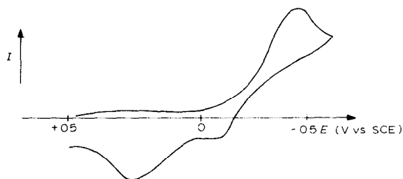
Fig. 1. Cyclic voltammogram of [\text{Co}(\text{CO})_4]_3\text{SnCl} in 0.1 M TBAP DME solution with a hanging mercury drop cathode. Scan rate 50 \text{ mV s}^{-1}
