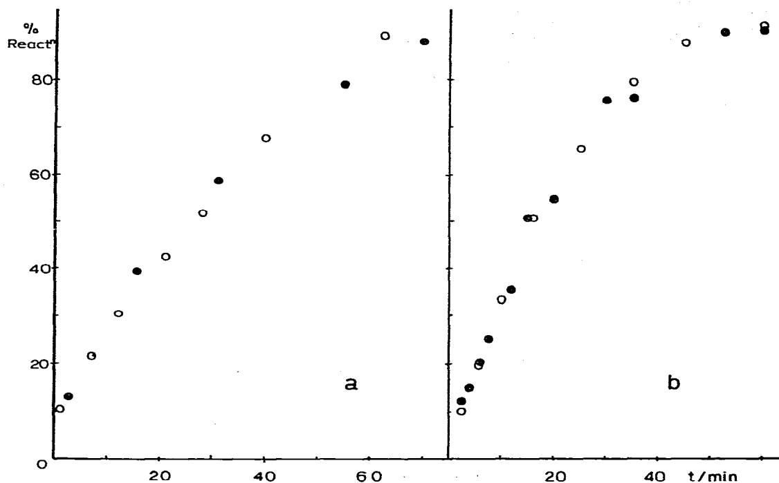
Fig. 1. Reproducibility of reactions. (a) [\text{EtOH}]_{\text{init}} , 0.294 \text{ mol dm}^{-3} ; [\text{HSi}(\text{OEt})_3]_{\text{init}} , 0.717 \text{ mol dm}^{-3} ; catalyst, 0.7 g batch VI (0.044 mmol Ir); solvent, toluene; temperature, 40^\circ\text{C} . (b) [\text{Ph}(\text{CH}_2)_2\text{OH}]_{\text{init}} , 0.147 \text{ mol dm}^{-3} ; [\text{PS50}]_{\text{init}} , 0.717 \text{ mol}(\text{Si-H}) \text{ dm}^{-3} ; catalyst, 0.7 g batch III (0.055 mol Ir); solvent, toluene; temperature, 40^\circ\text{C} .
