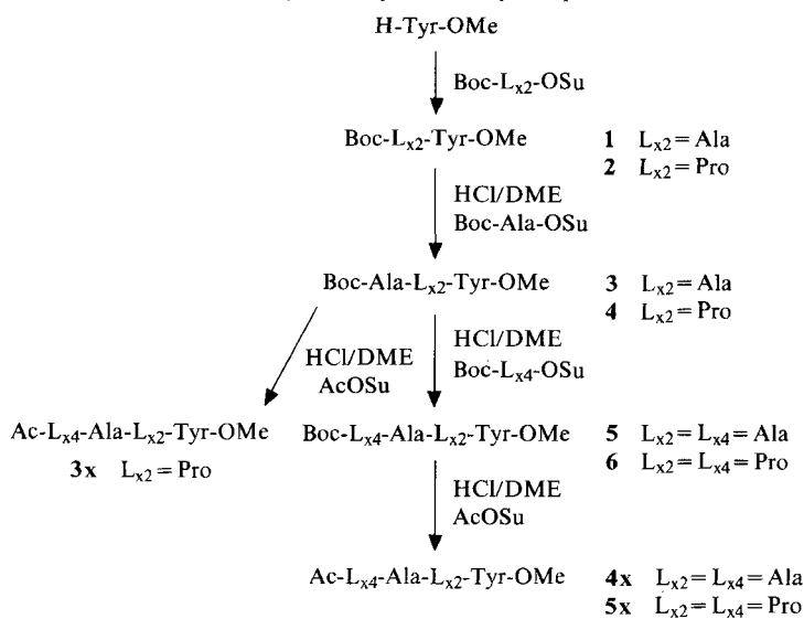
Scheme 3. Synthesis of the carboxyl components X-A
