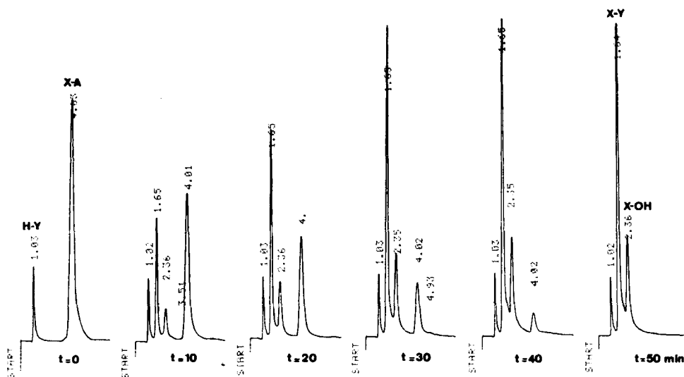
Fig. 1. Progress of \delta -chymotrypsin-catalyzed synthesis of 3x-1y monitored by HPLC. (X-A = 3x , H-Y = 1y and X-OH = 3x' )
