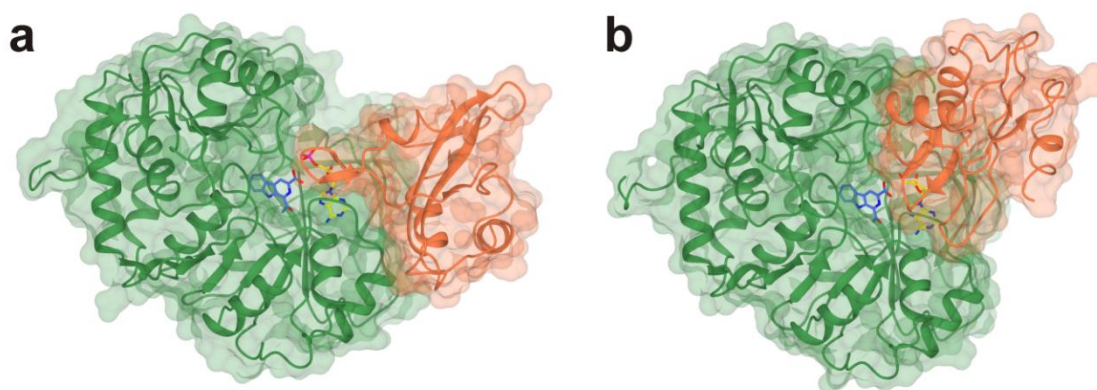
Figure 1. Structures of McbA in the adenylation (a) and amidation (b) conformations. In each case the protein is coloured in green from residues 1-394 (McbA N ) and coral from 395-494 (McbA C ). AMP (yellow) is bound at the domain interface and 6 (blue) within a binding pocket in the N-terminal domain. The McbA C domain in b is rotated 149° relative to the larger McbA N domain compared with their orientations in a .
