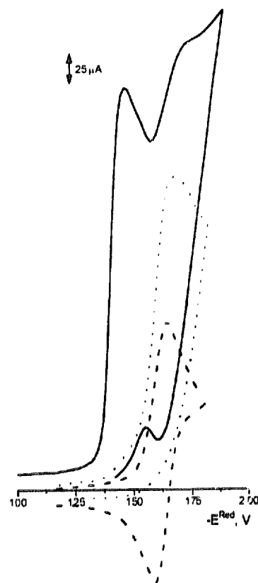
Fig. 2. Cyclic voltammograms obtained at an Hg electrode in \text{CH}_3\text{CN} with 0.05 M n\text{-Bu}_4\text{NBF}_4 as a supporting electrolyte: (a) 5 \times 10^{-4} M o -dicyanobenzene (—); (b) a mixture of 3 \times 10^{-3} M iodobenzene and 5 \times 10^{-4} M o -dicyanobenzene (---); (c) the same as (b) on addition of 3 \times 10^{-3} M [\text{CpFe}(\text{CO})_2]_2 (.....). The reference electrode was aqueous \text{Ag}/\text{AgCl}/\text{KCl} , the scan rate was 200 \text{ mV s}^{-1} .
