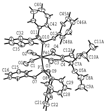
Fig. 2. ORTEX diagram of the molecular structure of 4c (major conformation). Selected bond lengths (Å) and angles (°): Fe–P1, 2.1631(12); Fe–P2, 2.1747(12); Fe–C1, 1.812(4); Fe–C2, 1.773(8); Fe–C3, 1.959(7); Fe–C6, 2.004(5); C3–C4, 1.520(6); C4–C5, 1.321(7); C5–C6, 1.503(7); C3–O3, 1.247(6); C6–O4, 1.222(6); P1–Fe–P2, 167.89(4); C1–Fe–C2, 97.4(2); C2–Fe–C6, 91.6(3); C3–Fe–C6, 80.8(2); C1–Fe–C3, 90.3(2); Fe–C6–C5, 113.8(4); Fe–C3–C4, 115.4(5).
