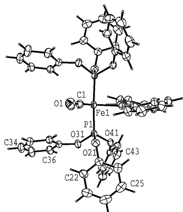
Fig. 1. ORTEX diagram of the molecular structure of 3a . Selected bond lengths (Å) and angles (°): Fe–P1, 2.1702(5); Fe–C1, 1.769(2); Fe–C2, 2.0566(16); C2–C2', 1.274(4); C2–C11, 1.447(3); P1–Fe–P1, 177.04(2); C1–Fe–C1, 111.06(12); C1–Fe–C2, 142.35(8); C2–Fe–C2, 36.10(11); Fe–P1–O21, 112.20(5); Fe–P1–O31, 120.58(6); Fe–P1–O41, 118.20(5). Symmetry operator ' = -x, y, 1/2 - z .
