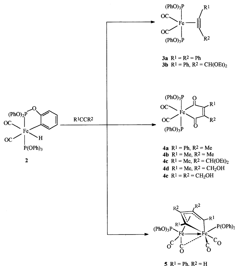
Scheme 1. Reactions of \text{HFe}(\text{CO})_2\{\text{P}(\text{O}^i\text{Ph})_3\}\{(\text{PhO})_2\text{POC}_6\text{H}_4\} ( 2 ) with alkynes \text{R}^1\text{CCR}^2 .
